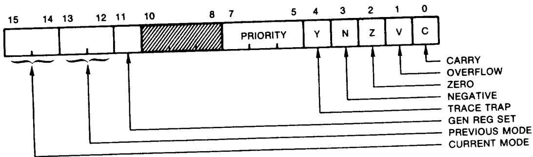
Figure B-1 Format of the Processor Status Word
