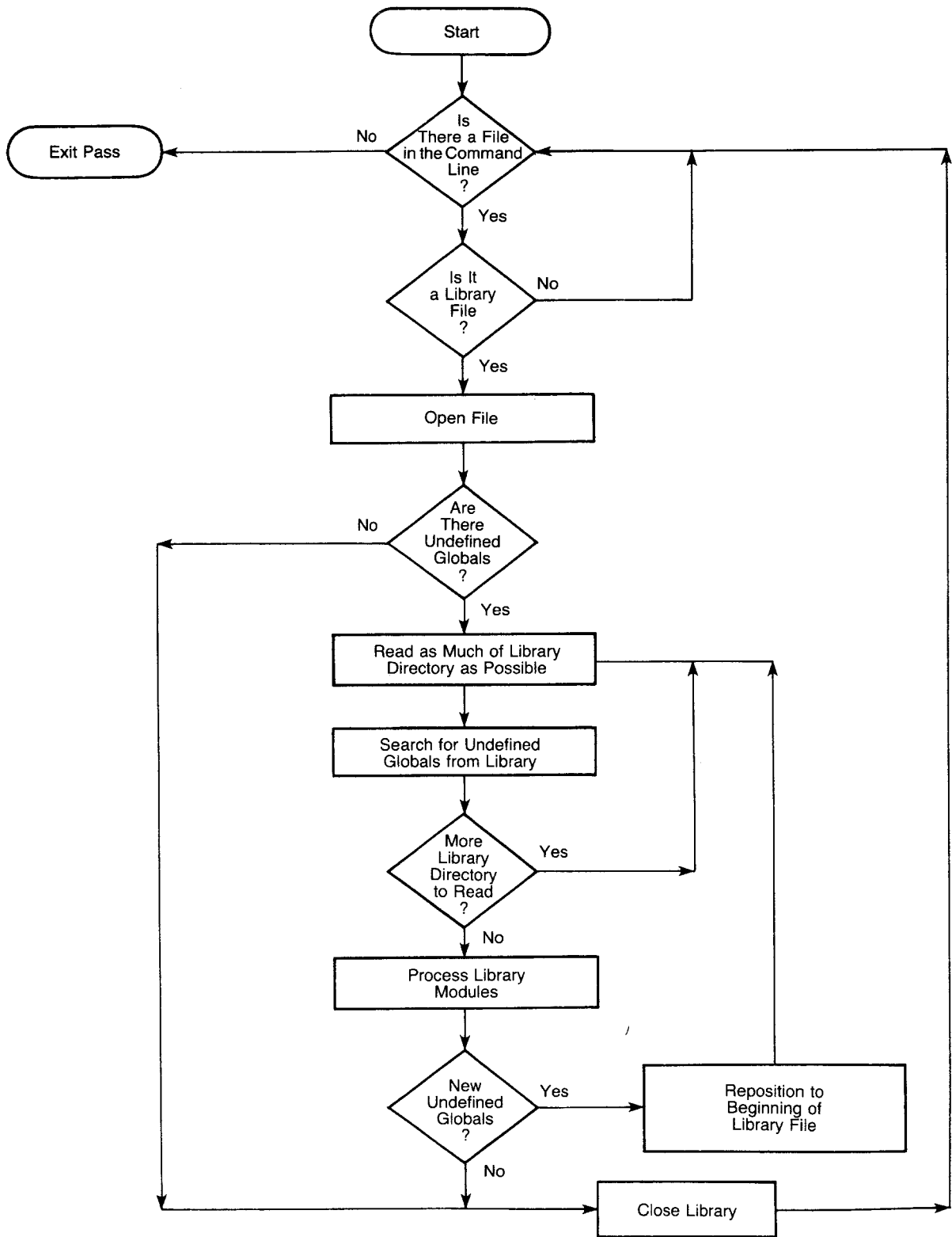
Figure 3-1: Library Searches
